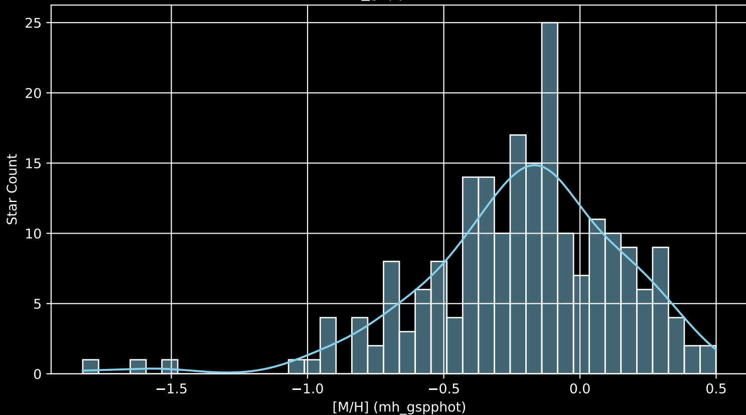
APOGEE DR17 Field: [081+53_MGA [M/H] (mh_gspphot) (n= 209)
