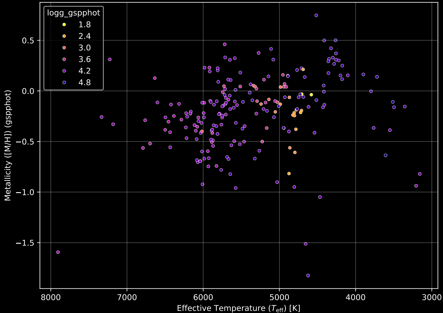
APOGEE DR17 Field: [081+53_MGA] Stellar Population Parameters (n= 211)
