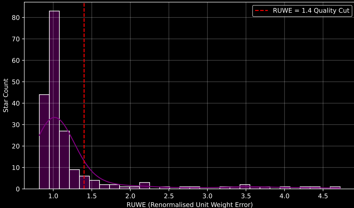
GAPOGEE DR17 Field [081+53_MGA] RUWE Distribution (n= 195)
