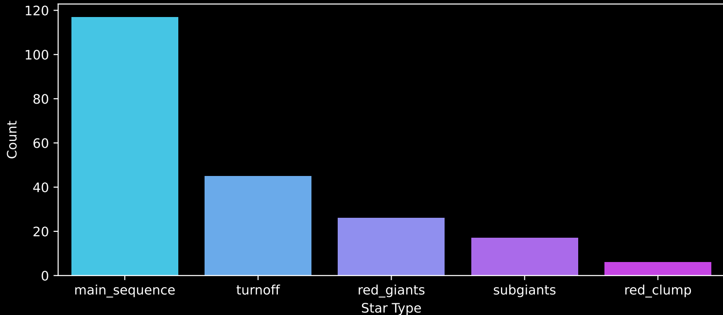
APOGEE DR17 Field: [081+53_MGA] Count plot of Star Type
