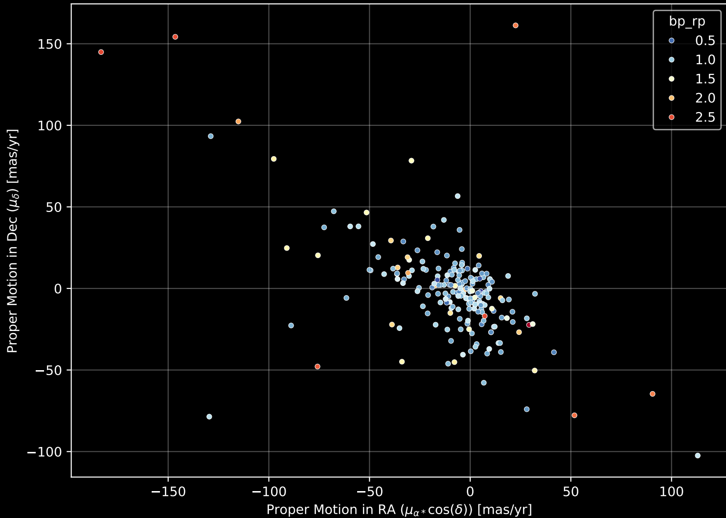
APOGEE DR17 Field: [081+53_MGA] Proper Motion Diagram (n= 211)
