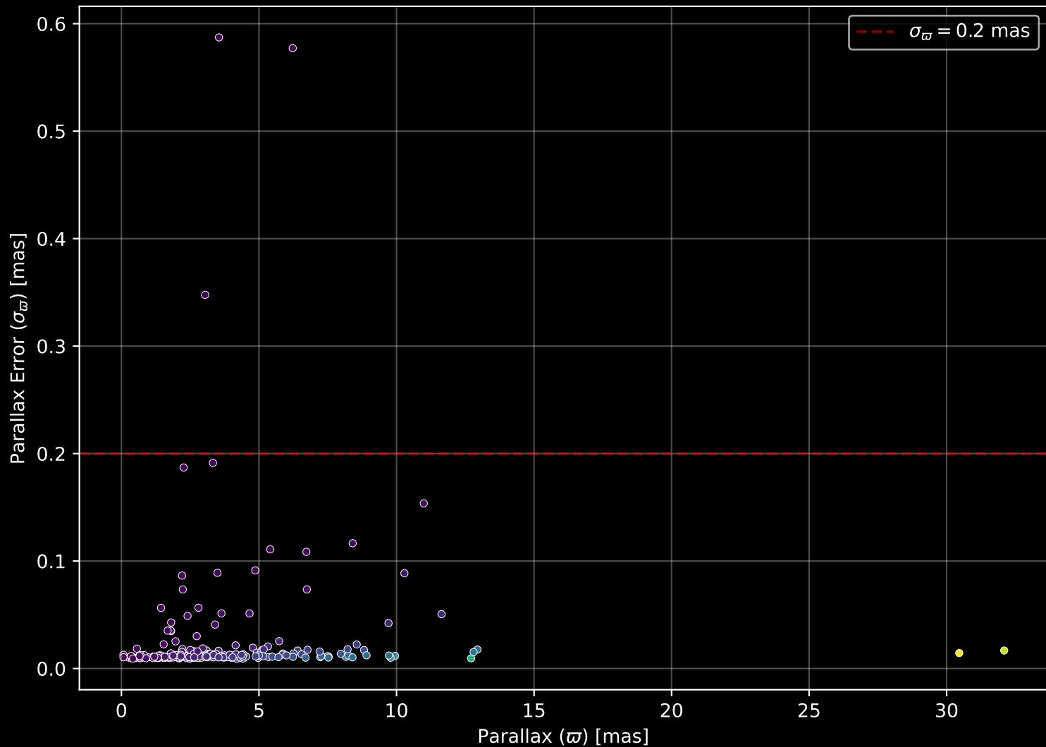
APOGEE DR17 Field: [081+53_MGA] Parallax Quality (n= 211)
